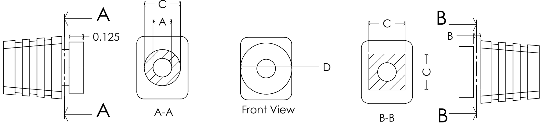
Round Slot
