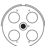
32-79 1-#8; 4-#4 ● ⊙ D
