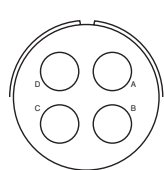
LAYOUT # OF CONTACTS 4-#4 (coax) RG-161/U or RG-179/U SERIES ● ⊙ SERVICE RATING (coax)
