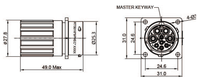
Sqaure Flange Receptacle with Endcap
