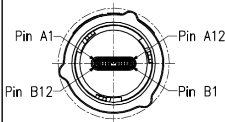
Conn.1 Pin Assignments Front View
