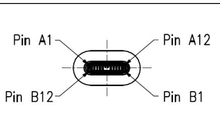
Conn.2 Pin Assignments Front View
