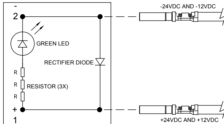
LED CONNECTOR DIAGRAM
