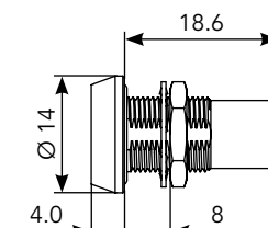
Front Mount Extended (HH)
