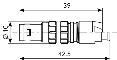
Straight Plug (FD)*
