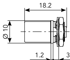
Protruding Front Mount (ED)
