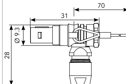
Right Angle Plug with Lanyard (FM) *
