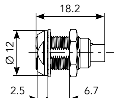
Double Nut (EA)
