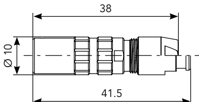
In Line Cable Receptacle (PC)*
