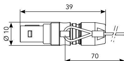
Straight Plug with Lanyard (FN) *
