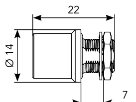
Protruding Front Mount (HD)
