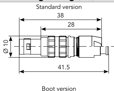
Straight Plug (FH)*
