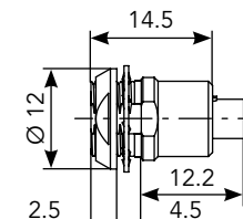
Rear Mount (EP)
