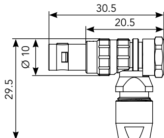
Right Angle Plug (FC)*
