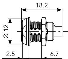
Double Nut (EA)
