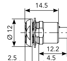
Rear Mount (EP)
