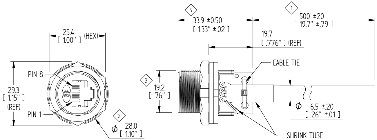
RJ45 JACK
